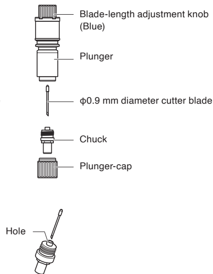
PHP35-CB09-HS φ0.9 mm diameter cutter Plunger
