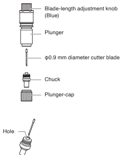
PHP35-CB09-HS φ0.9 mm diameter cutter Plunger
