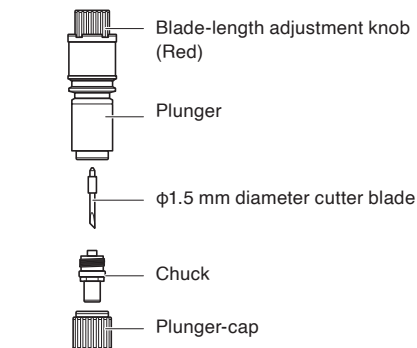
\phi 1.5 mm diameter cutter Plunger
