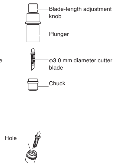
PM-CH-001 φ3.0 mm diameter cutter Plunger
