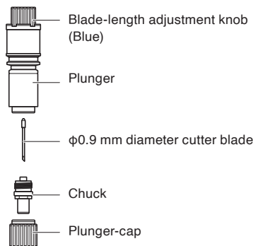
\phi 0.9 mm diameter cutter Plunger
