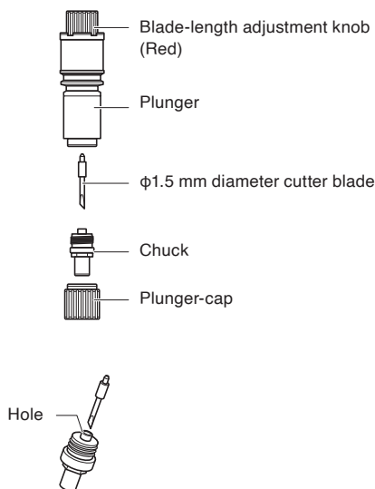
PHP35-CB15-HS φ1.5 mm diameter cutter Plunger
